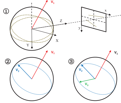
Figure 3. Procedures of how to generate three orthogonal vanishing points. The first vanishing point \mathbf{v}_1 is the intersection point of two line segments, \mathbf{v}_2 is uniformly sampled on the great circle of \mathbf{v}_1 , and \mathbf{v}_3 is the cross product of \mathbf{v}_1 and \mathbf{v}_2 .
