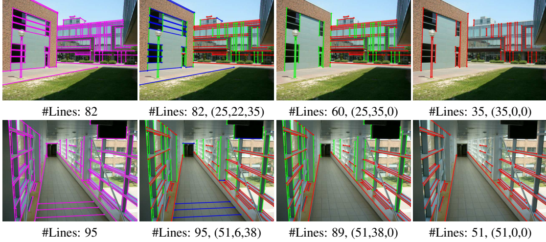
Figure 6. Vanishing point estimation results of the proposed method on the YUD dataset with 3, 2, and 1 vanishing point(s). The triple “( , , )” denotes the numbers of line segments corresponding to different vanishing points, respectively.
