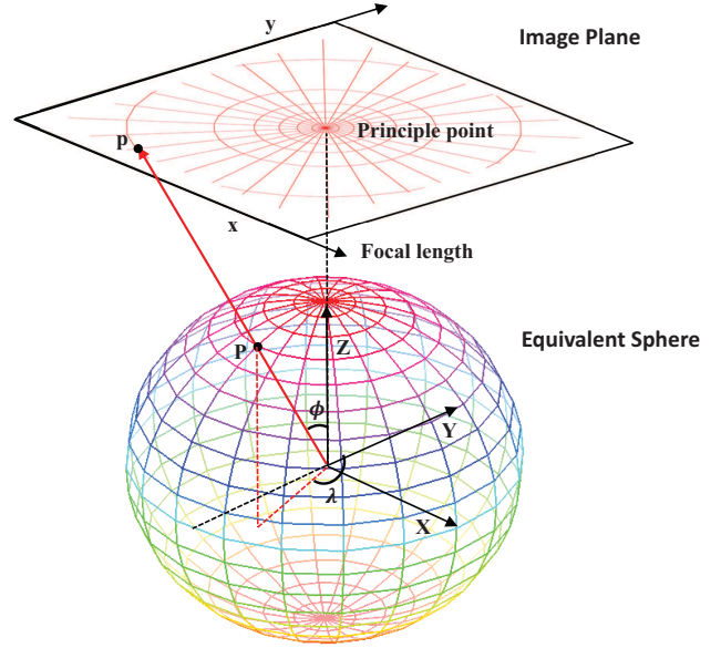
Figure 2. Demonstration of the relationship between the image plane and the equivalent sphere, and the procedure of how to build the polar grid. Notice that only the hemisphere toward the image plane is projected onto the image plane.
